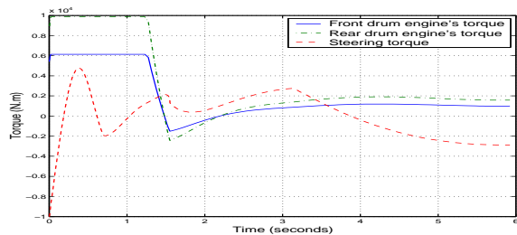
Fig. 5. Actuator torques for the base motion
