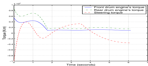
Fig. 6. Actuator torques for the optimized motion
