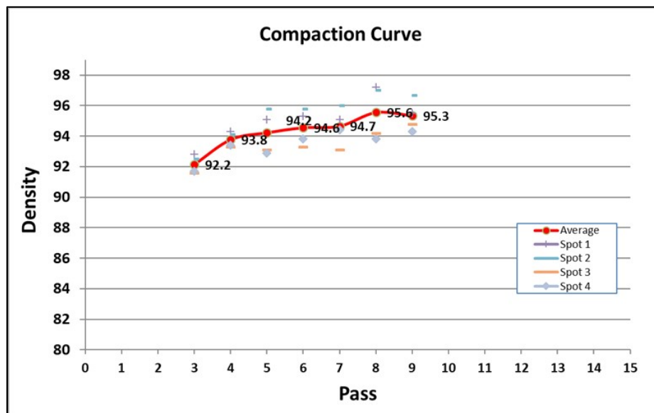
Figure 51: Trial Section Compaction Curve J113169, I-35.
