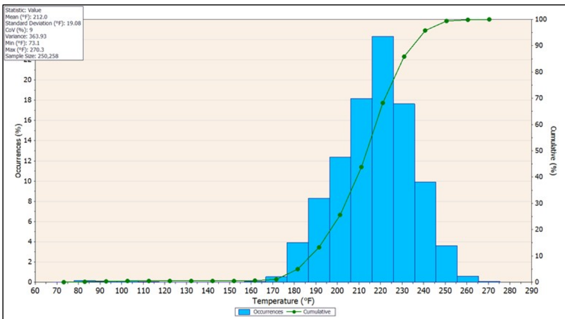
Figure 48: Veta Temperature Statistics Screen of IC Data Analysis J6I3189, I-44.
