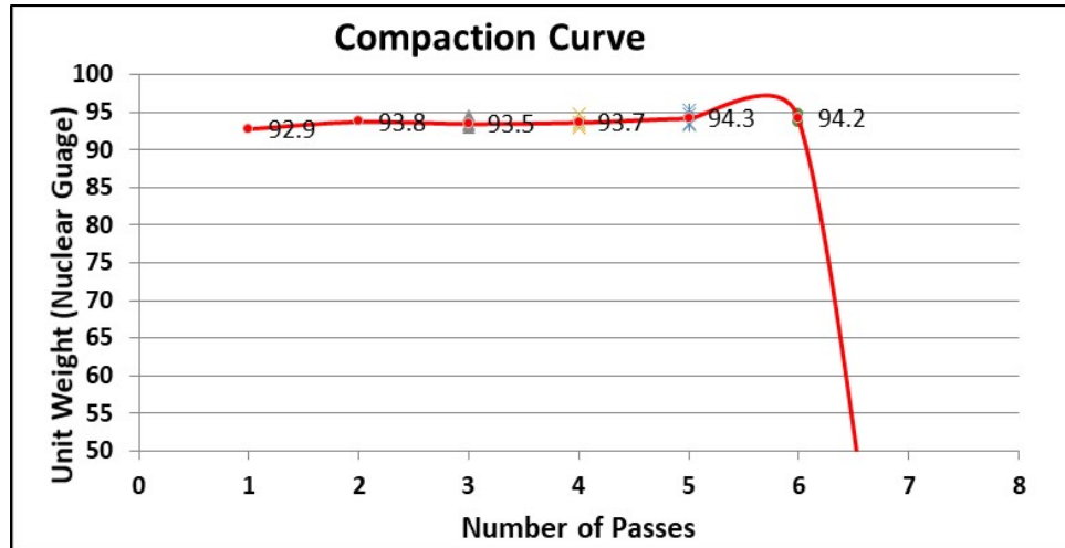
Figure 77: Trial Section Compaction Curve for J6P3184, Rte. 141.
