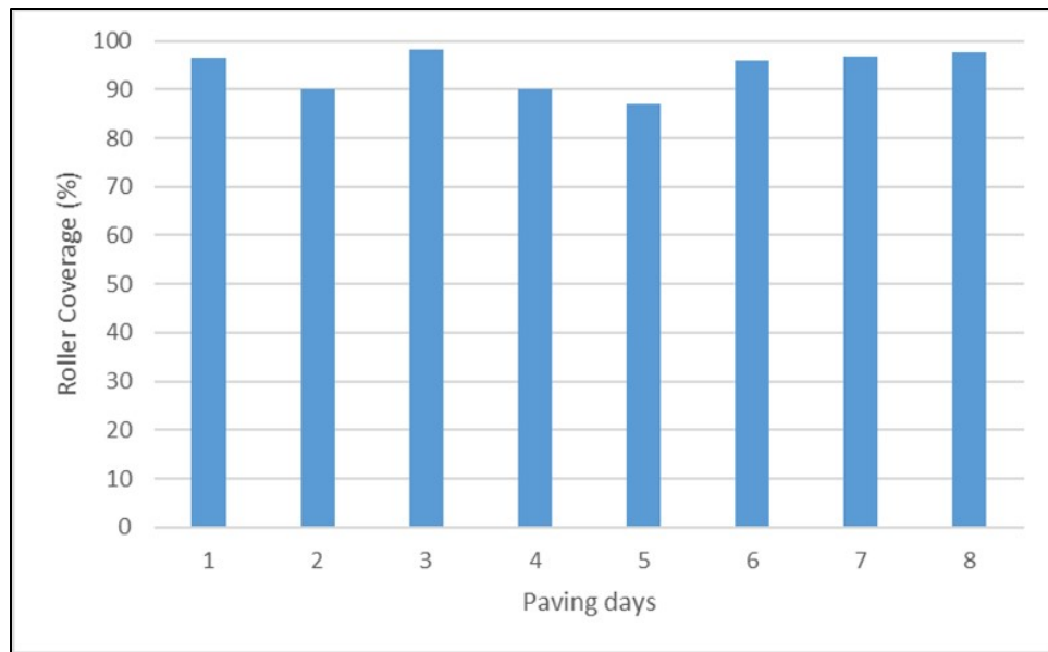
Figure 79: Summary of Roller Coverage Report for J6P3184, Rte. 141.
