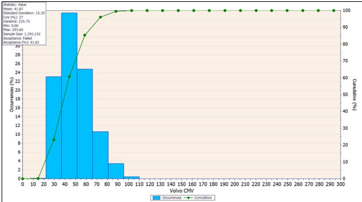
Figure 47: Veta CMV Statistics of IC Data Analysis J6I3189, I-44.
