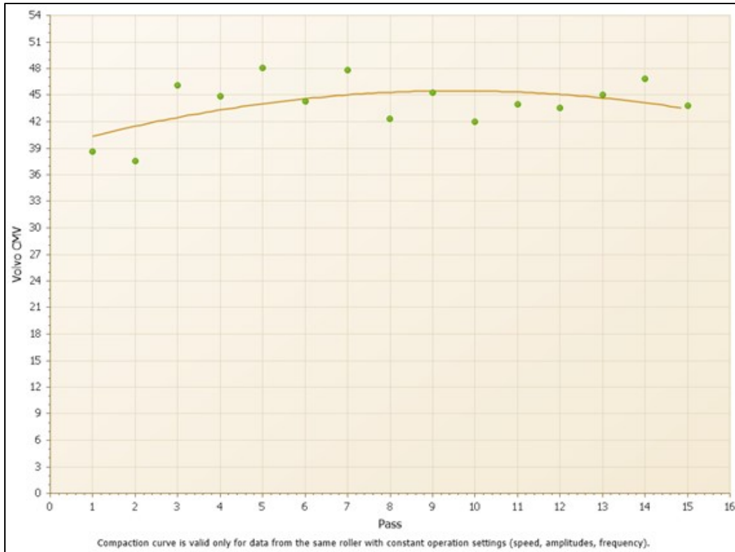
Figure 43: Veta Compaction Curve Screen of IC Data Analysis J6I3189, I-44.
