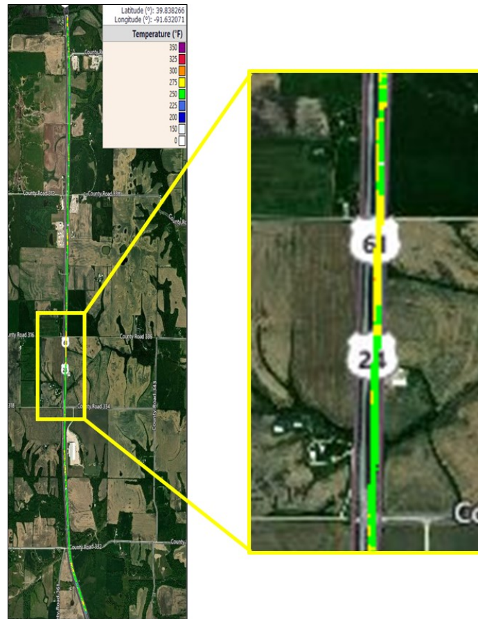
Figure 15: RoadScan PMTPS Data in Veta (HWY 61/24 Project).
