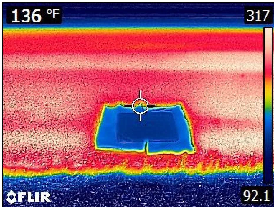
Figure 24. Photo. Improvised reference object met the dimensions required and stayed below 150°F during testing.
