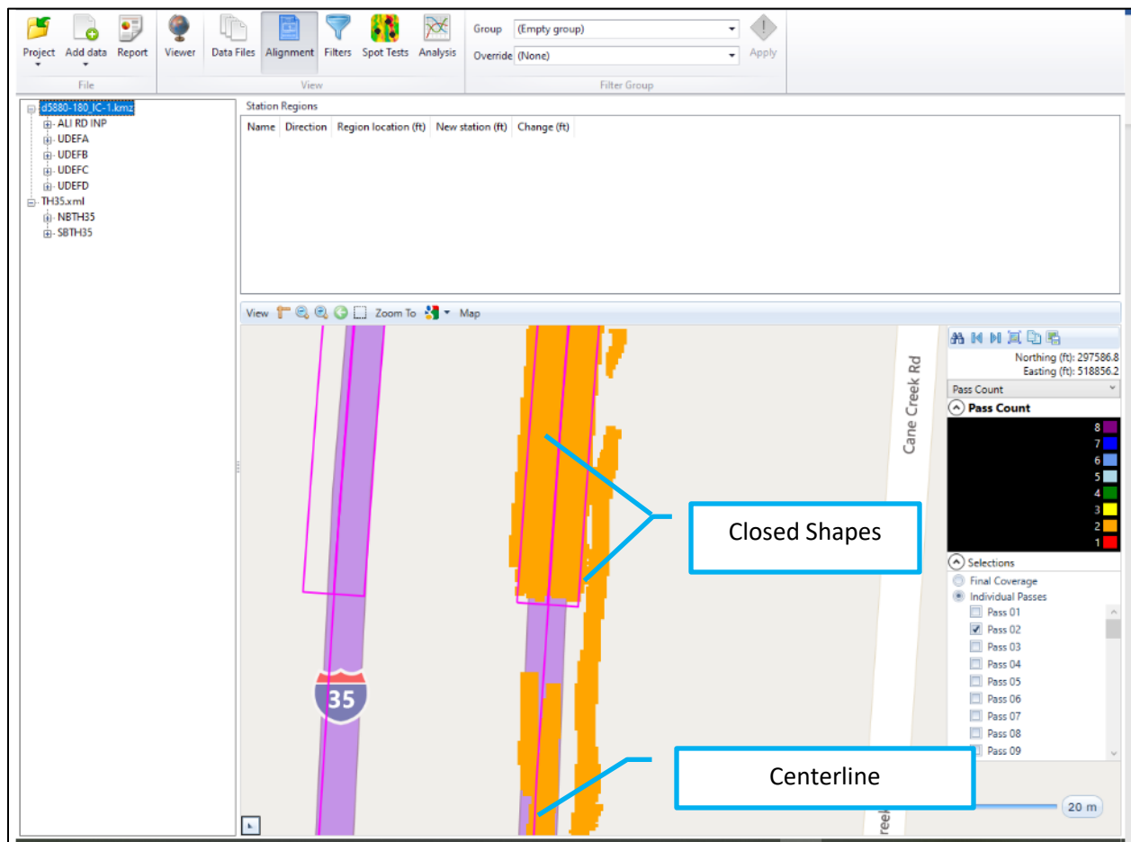
Figure 23. Available elements in an example .kmz alignment file.
