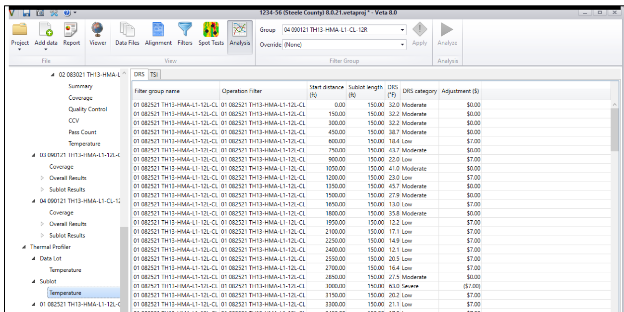
Figure 111. Sublot temperature results.
