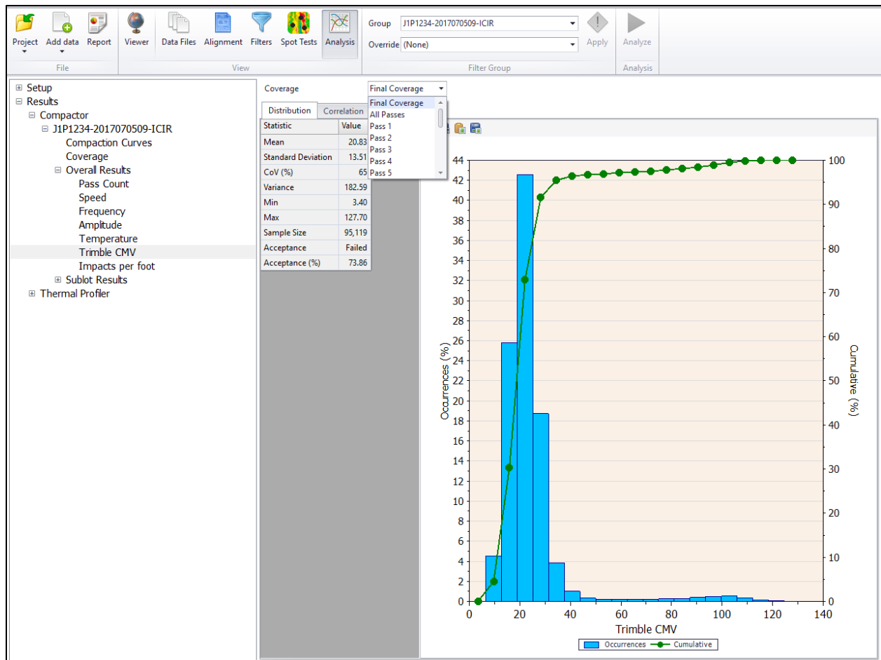
Figure 101. Overall results for ICMV.
