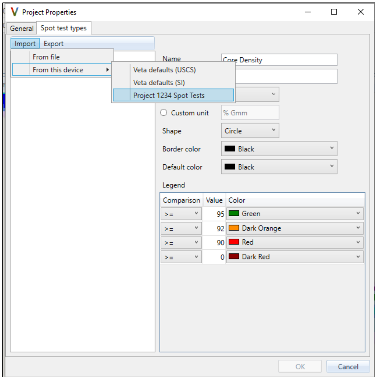
Figure 81. Spot tests can be assigned to the project under Project → Properties.
