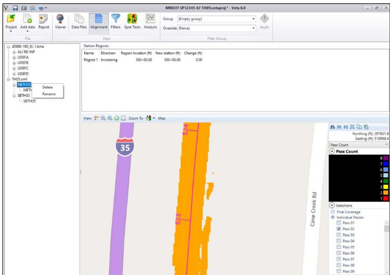
Figure 26. The alignment screen can be used to identify different elements in alignment files. Elements can be renamed or deleted by right-clicking on the element.
