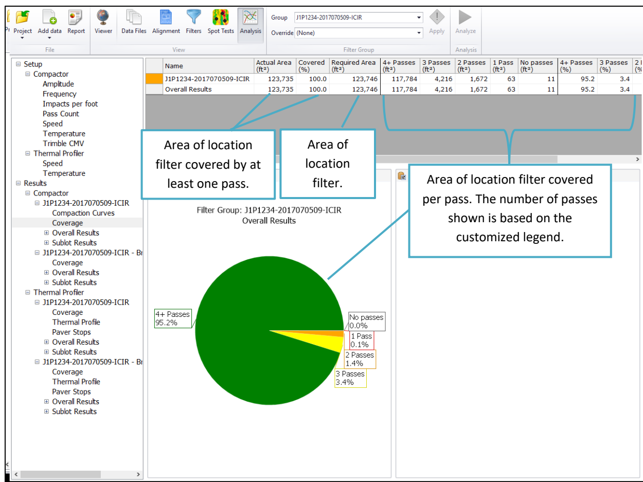
Figure 100. Coverage results.
