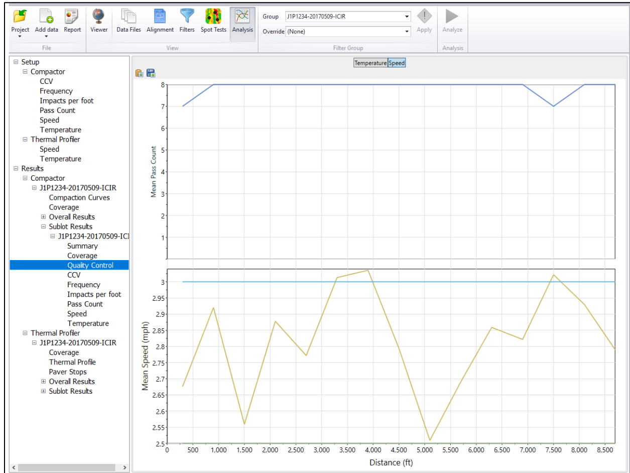
Figure 106. Sublot quality control results for the mean speed.
