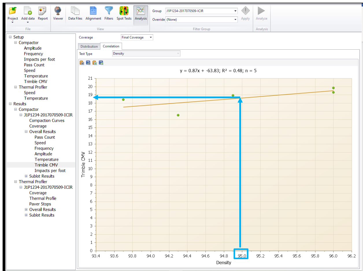
Figure 102. Correlation curve showing the relationship between core density data and ICMV.
