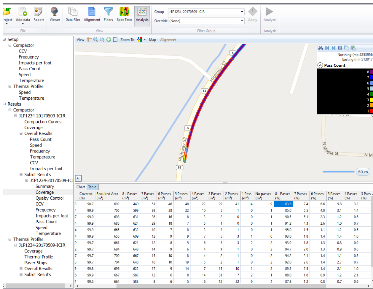
Figure 105. Subplot coverage results.
