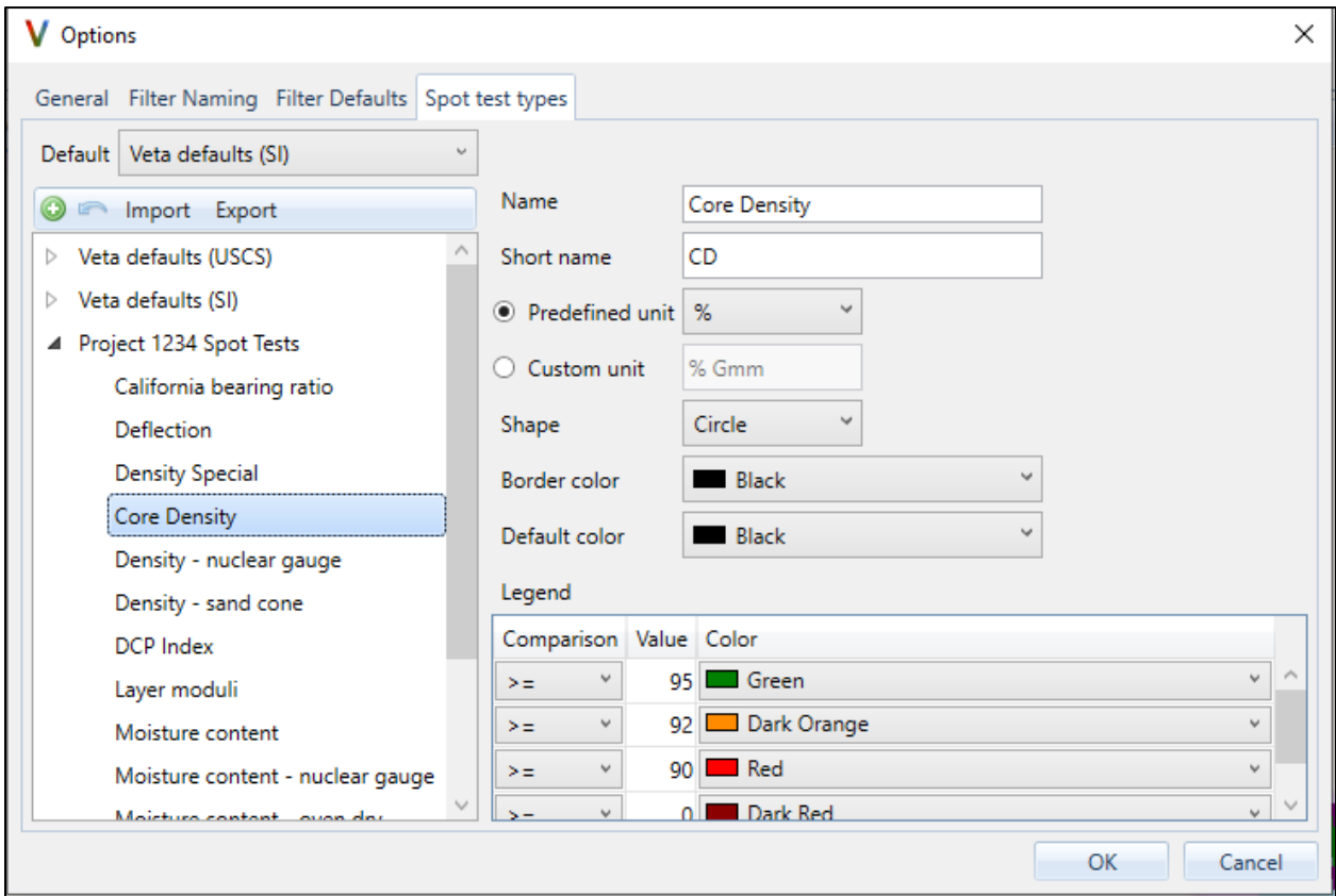
Figure 80. Default spot test types can be customized under “options.”
